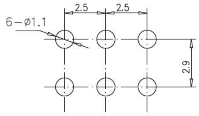
PWB mounting hole for reference
