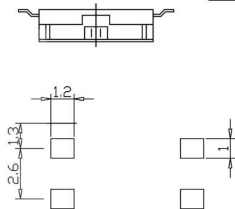
Pad Layout
