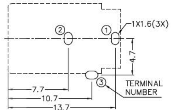
RECOMMENDED PCB LAYOUT TOLERANCE: ±0.05 (TOP VIEW)
